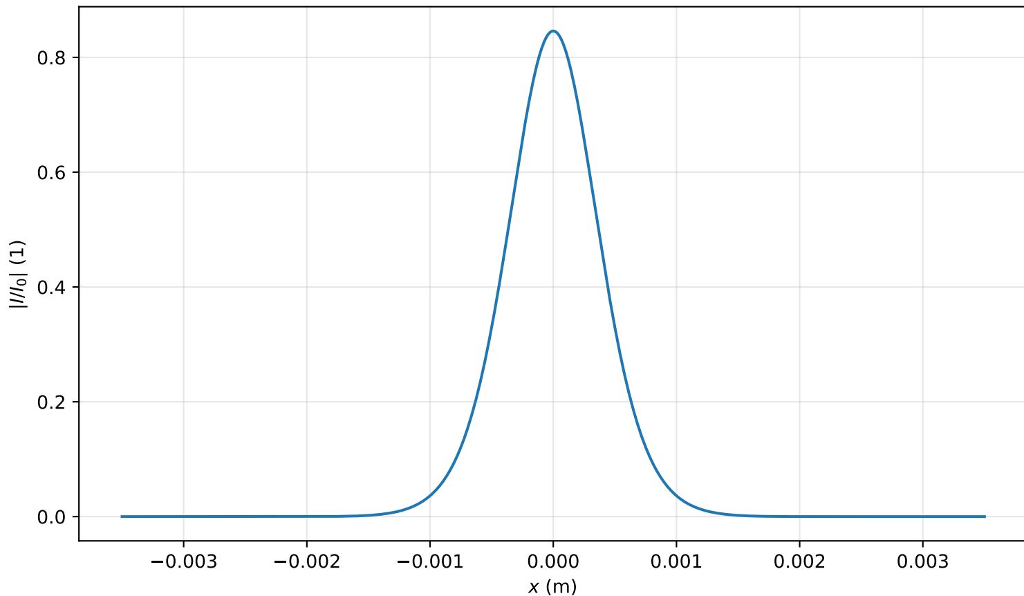
Intensity profile I(x, y = 0, z = 1.592m)/I_0 , P_{in}=0.4P_{cr} , artificial time
